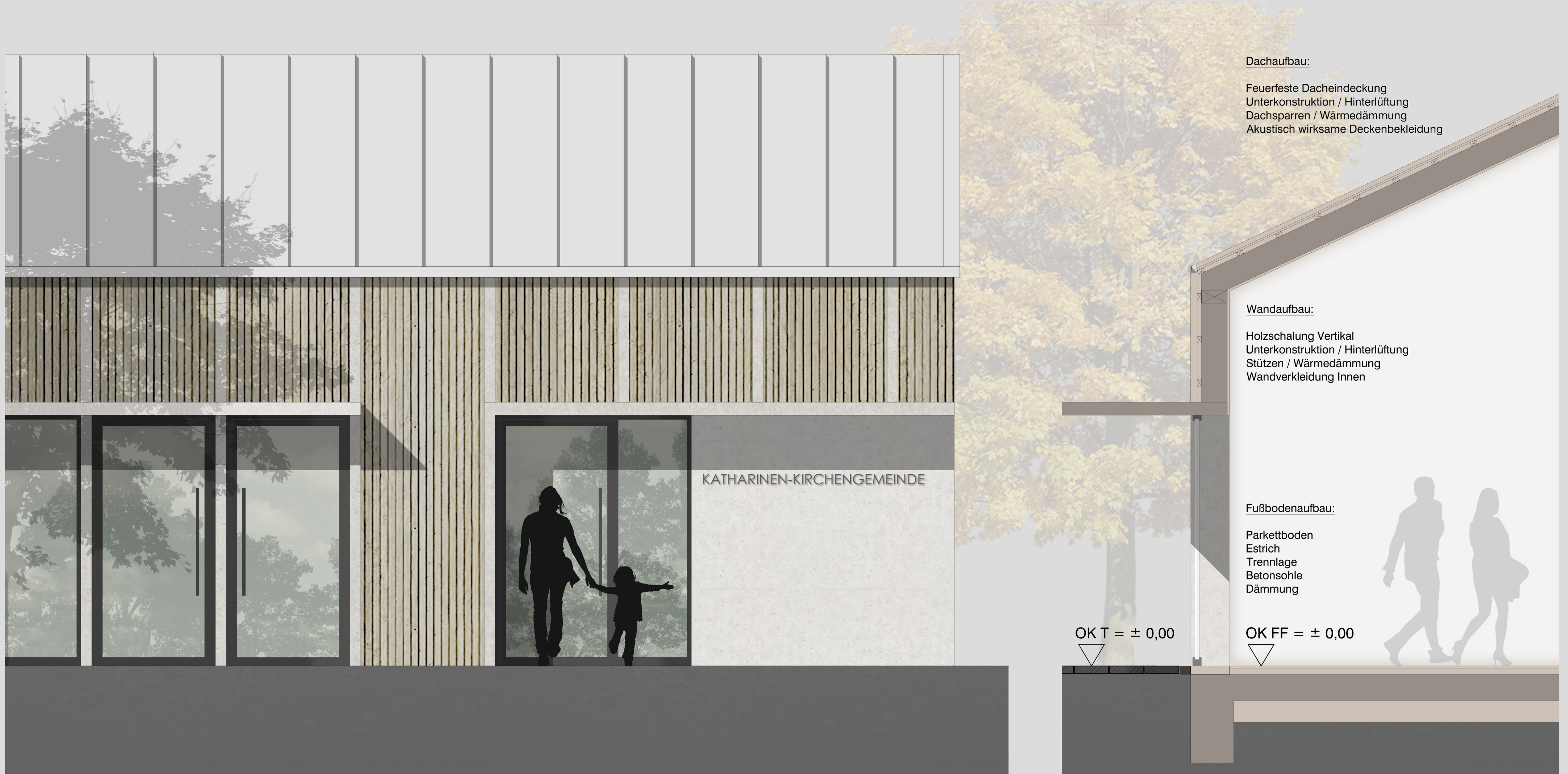
DETAIL M 1:25
